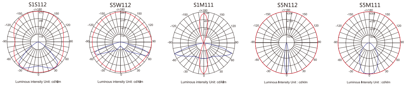
Light Distribution Curve
