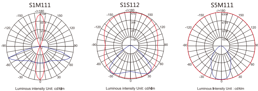
Light Distribution Curve
